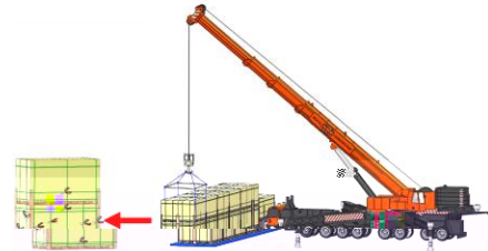
Vertical landscape package unloading with crane
